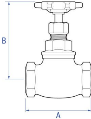
1031 Globe valve
