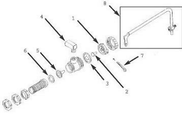
858N-Z Float valve
