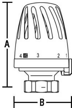
B1301 Liquid head
