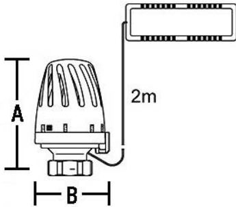
B1401 Liquid head with remote sensor
