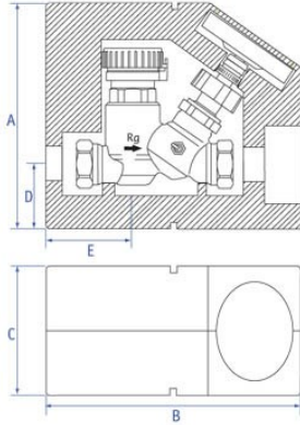
Insulation jacket for circulating valves
