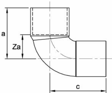
NS12S/5092 Elbow
