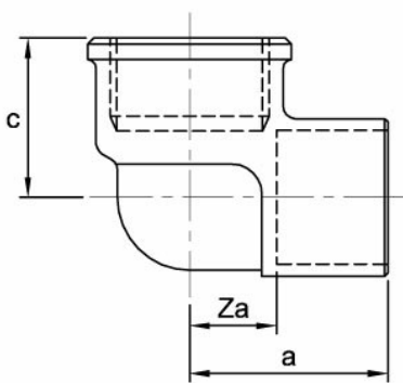
N14/4090G Elbow
