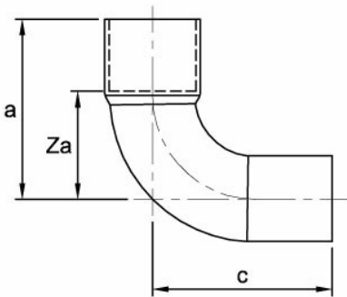
N18S/5001A Elbow
