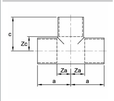
N24/5130 Tee
