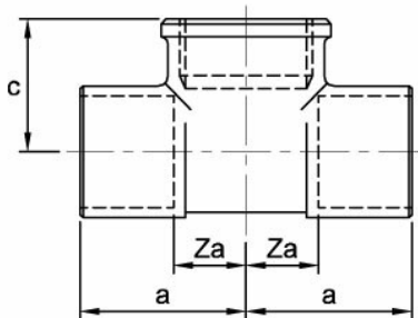
N30/4130G Tee
