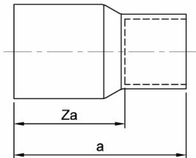
N6/5243 Reducer
