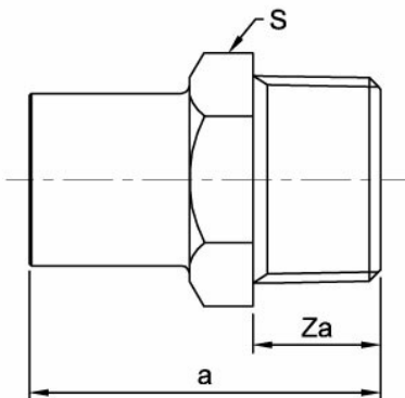
N8/4280G Adaptor
