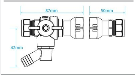
PB360WMK Water meter kit
