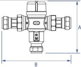
PEG402 Thermostatic mixing valve TMV3/2
