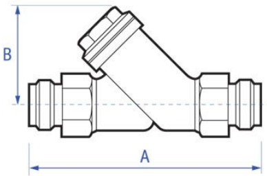
PT913 Strainer
