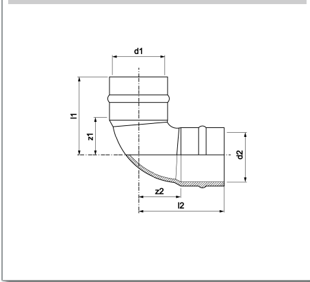
YP12 Elbow
