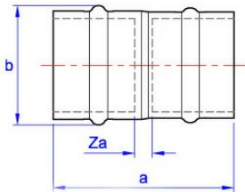
YP11M Slip Coupling
