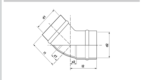
YP21 Elbow
