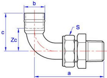
YP65 Connector
