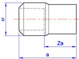
YP9B Adaptor
