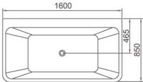
K1587 1600x850x570mm
