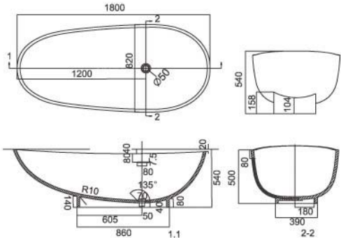
K1801 1800x820x540mm
