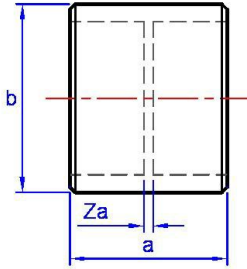
1GHD Coupling
