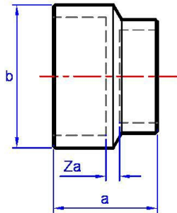
1RGHD Coupling
