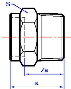
3GHD Connector
