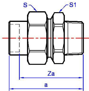
69GHDDW Connector
