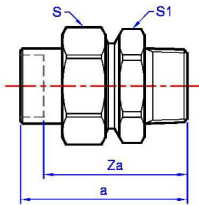
69GHD Connector
