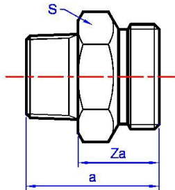
70GHD Nipple
