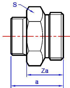
70PGHD Nipple
