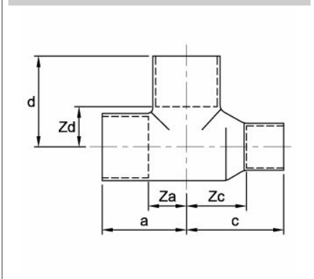
N26/5130 Tee
