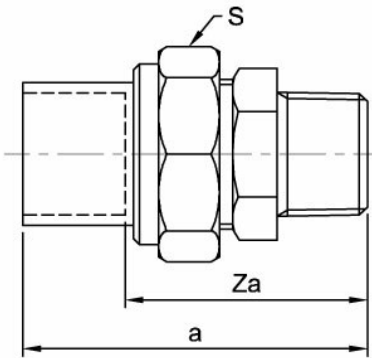
N69P Connector
