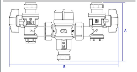
PEG402UA Thermostatic mixing valve TMV3/2
