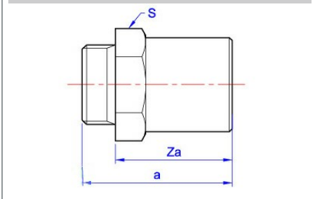
YP115 Nipple
