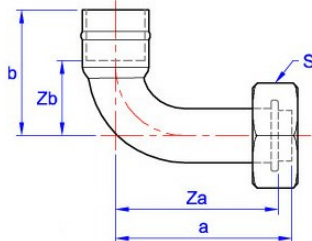
YP63L Connector
