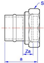
YP68M Connector
