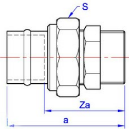
YP69F Connector
