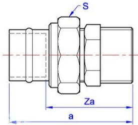
YP69P Connector
